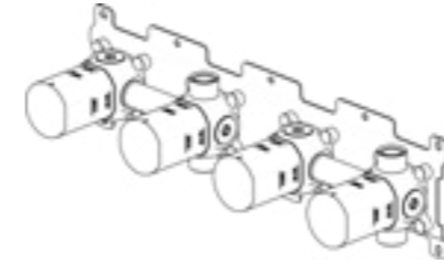
OIPIVA35022B Parte incasso per miscelatore vasca a parete Built-in part for floor washbasin mixer with shower kit
