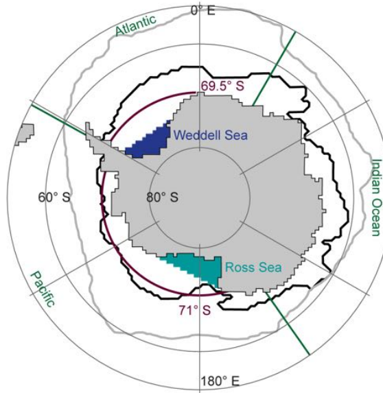
Figure 2.11 Regions used for evaluation of the sea-ice freshwater fluxes: Turquoise shading: area south of the coastal Ross Sea flux gate (Drucker et al., 2011; Kwok, 2005; Comiso et al., 2011); dark blue shading: area south of the coastal Weddell Sea flux gate (Drucker et al., 2011); purple lines: 69.5° S latitude band in the Atlantic sector and 71° S latitude band in the Pacific sector; black line: smoothed mean zero sea-ice-ocean freshwater flux line dividing the coastal and open ocean regions; thick gray line: mean sea-ice edge (1% sea-ice concentration); green lines: basin boundaries.
