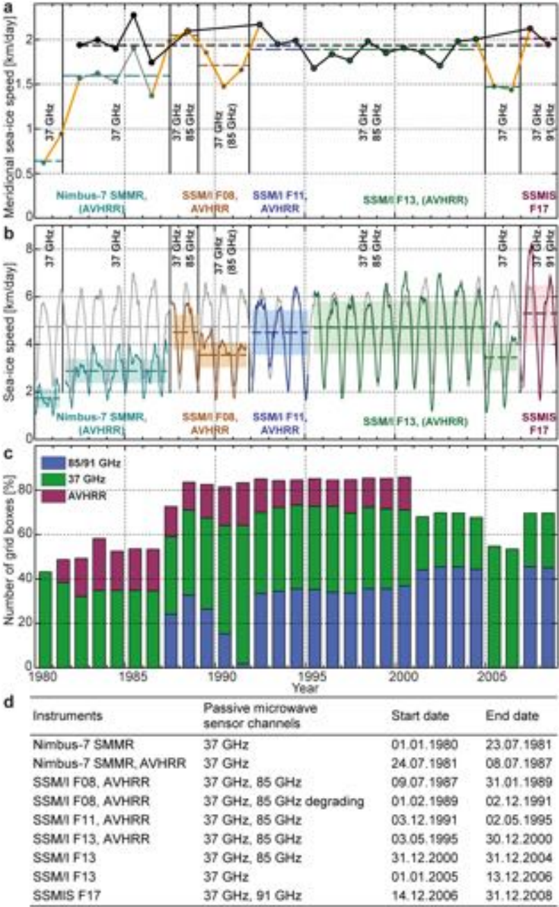
Figure 2.8 Temporal inhomogeneities in the NSIDC satellite sea-ice drift data: (a) Annual mean meridional sea-ice drift speed averaged over the entire sea-ice area (sea-ice concentration >50%). Thick orange lines: spurious trends due to changes in underlying data; black: data corrected for inconsistencies and used in this study (1982 to 2008). (b) Low-pass filtered (91-day running mean) sea-ice drift speed averaged over the entire sea-ice area (sea-ice concentration >50%). Gray: reduced wind speed from ERA-Interim using a reduction factor from the period 1988 to 2008. (a-b) In color: uncorrected data for each respective underlying satellite instrument combination; dashed lines: mean over the respective period; black vertical lines: periods of the same underlying channels. Text denotes the sensors and the frequency of the microwave radiometer channels used. (c) Fraction of sea-ice covered grid boxes with at least one drift vector observation in a 21-day window and a 75 by 75 km grid box using the non-gridded NSIDC drift data. Colors indicate the contribution of each sensor and channel. (d) Different combinations of instruments and passive microwave sensor channels and the related periods underlying the NSIDC sea-ice drift data.
