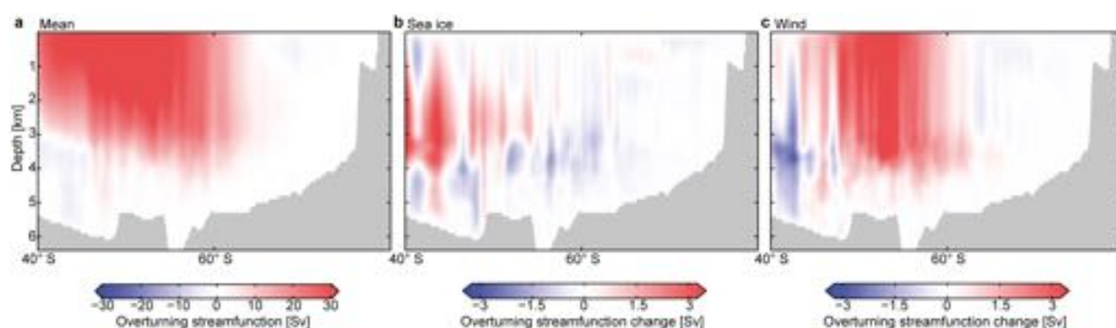
Figure 4.9 Zonal mean meridional overturning response: Mean of the simulated meridional overturning circulation (a), response to the combined sea-ice and land-ice freshwater flux perturbations (b), and response to the surface wind stress perturbation (c). The responses show the differences of the last 20 years of a 40-year perturbation experiment to a control simulation with constant forcing. Note that apparent vertical lines are artifacts from interpolating the transport from the model's \sigma -coordinates to depth-levels.
