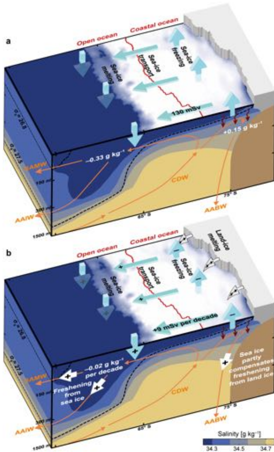
Figure 2.1 Effect of northward sea-ice freshwater transport on Southern Ocean salinity:
