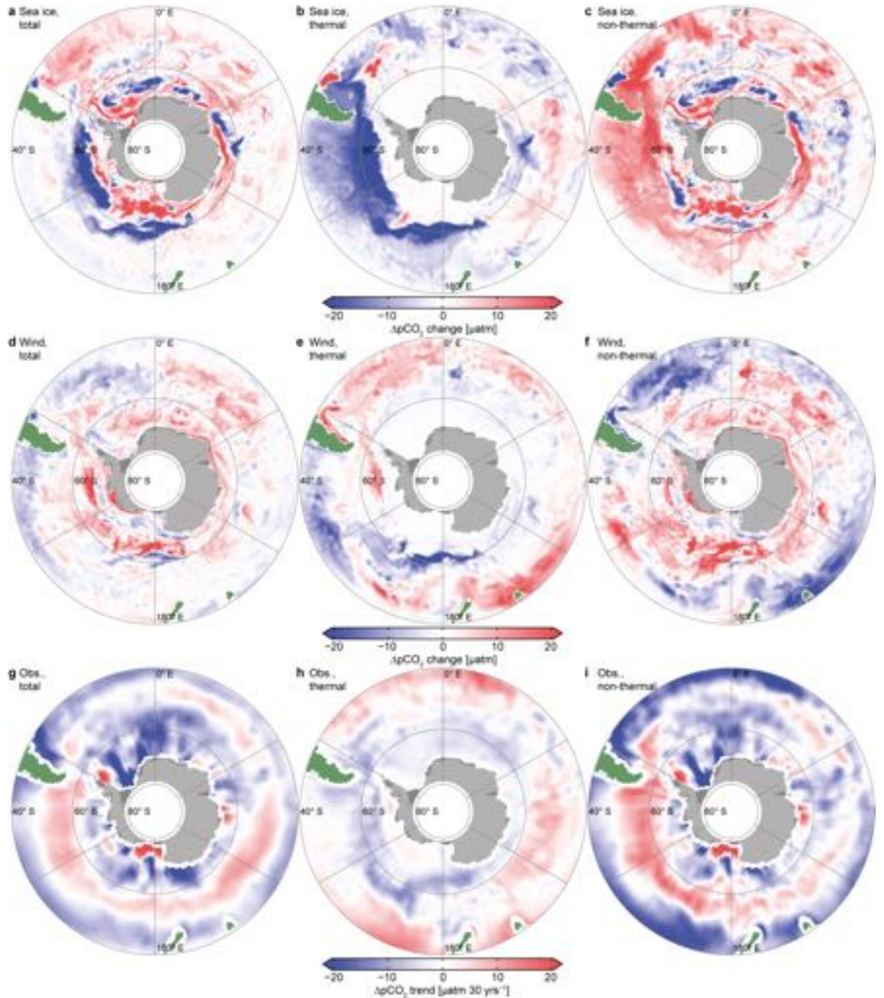
Figure 5.4 Observed and simulated \Delta p\text{CO}_2 changes and its thermal and non-thermal contributions: (a–c) Simulated \Delta p\text{CO}_2 change due to the sea-ice freshwater flux perturbation. (d–f) Simulated \Delta p\text{CO}_2 change due to the surface wind stress perturbation. (g–i) Observed trends derived from the period 1982–2014 Landschützer et al. (2015b, expanded as in Le Quéré et al. (2016)), scaled to a 30-year period. The middle column (b,e,h) shows the respective thermal contribution and the right column (c,f,i) the respective non-thermal contribution.
